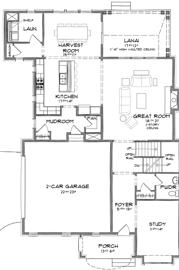
Main Level
